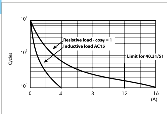
F 40.3 - Electrical life (AC) v contact current
