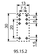
Copper side view
